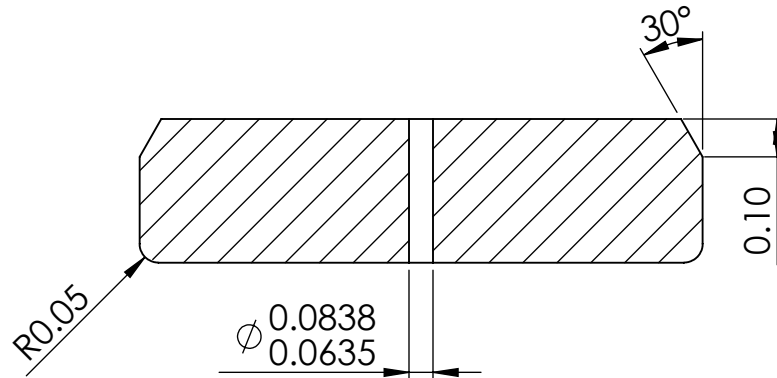
SECTION I-I
