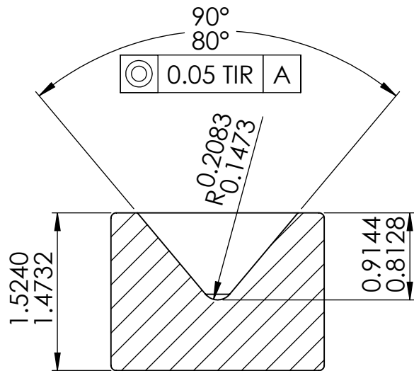
SECTION J-J
