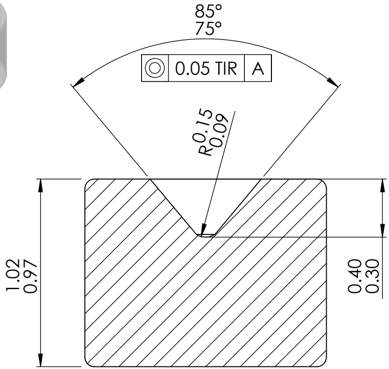
SECTION I-I
