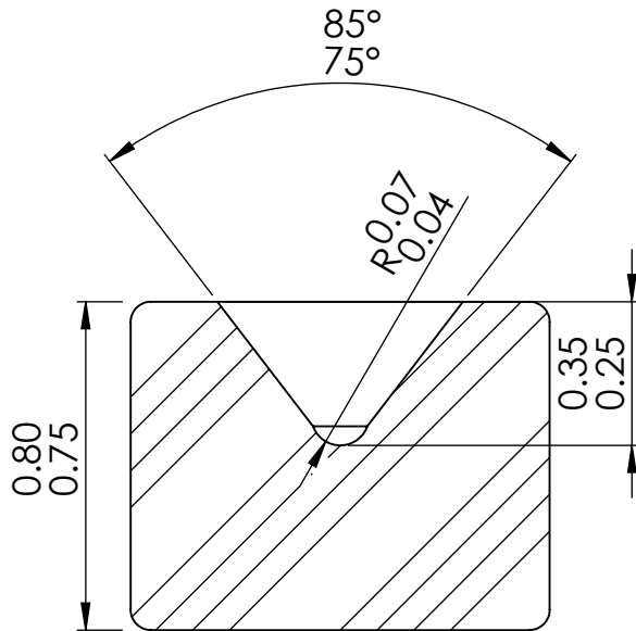
SECTION H-I
